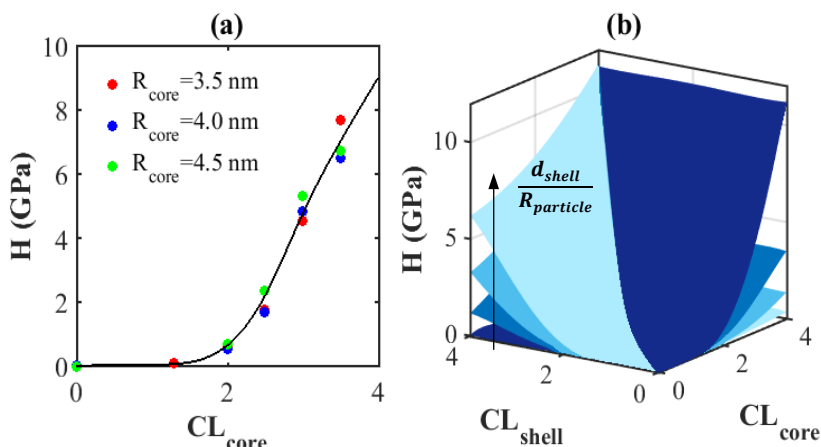
Figure 3. (a) H as a function of CL for particles without shell and with different sizes; (b) Surface plot for H as a function of CL in the core and in the shell at different core/shell ratio.
